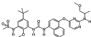
N-[5-tert-Butyl-2-methoxy-3-(3-{4-[2-(2-methoxy-1-methyl-ethylamino)-pyrimidin-4-yloxy]-naphthalen-1-yl}-ureido)-phenyl]-methanesulfonamide;
